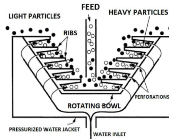
Schematic illustration of a Knelson Concentrator Source: Recovery of Silver From an Arsenical Silver Ore by Knelson Concentrator and Cyanide Leaching
